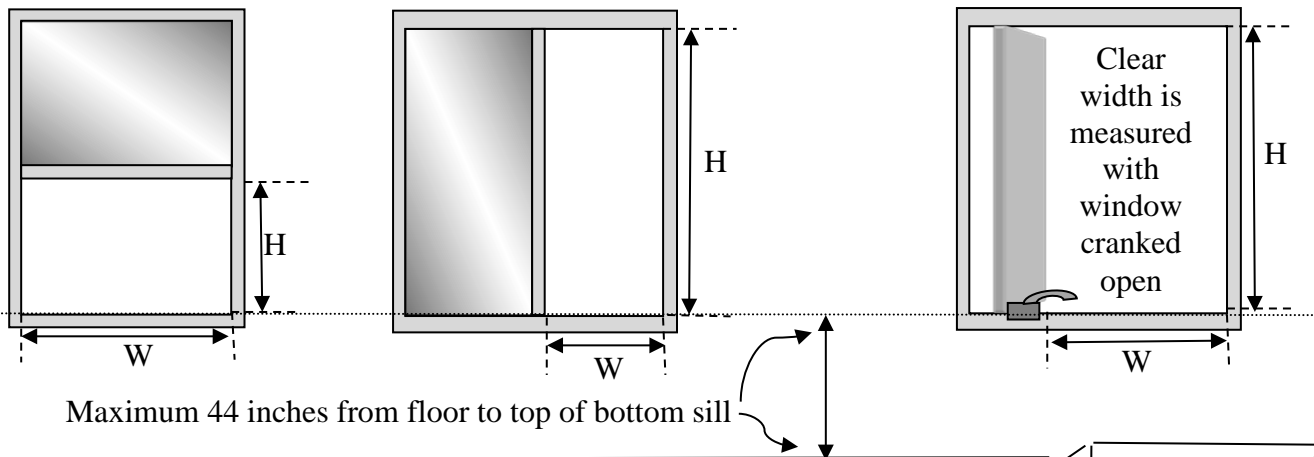
Single Hung Window
