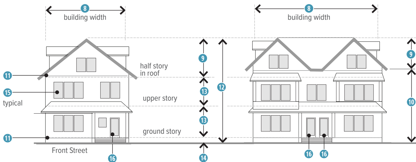
Figure 17. Cottage House Diagrammatic Elevation
