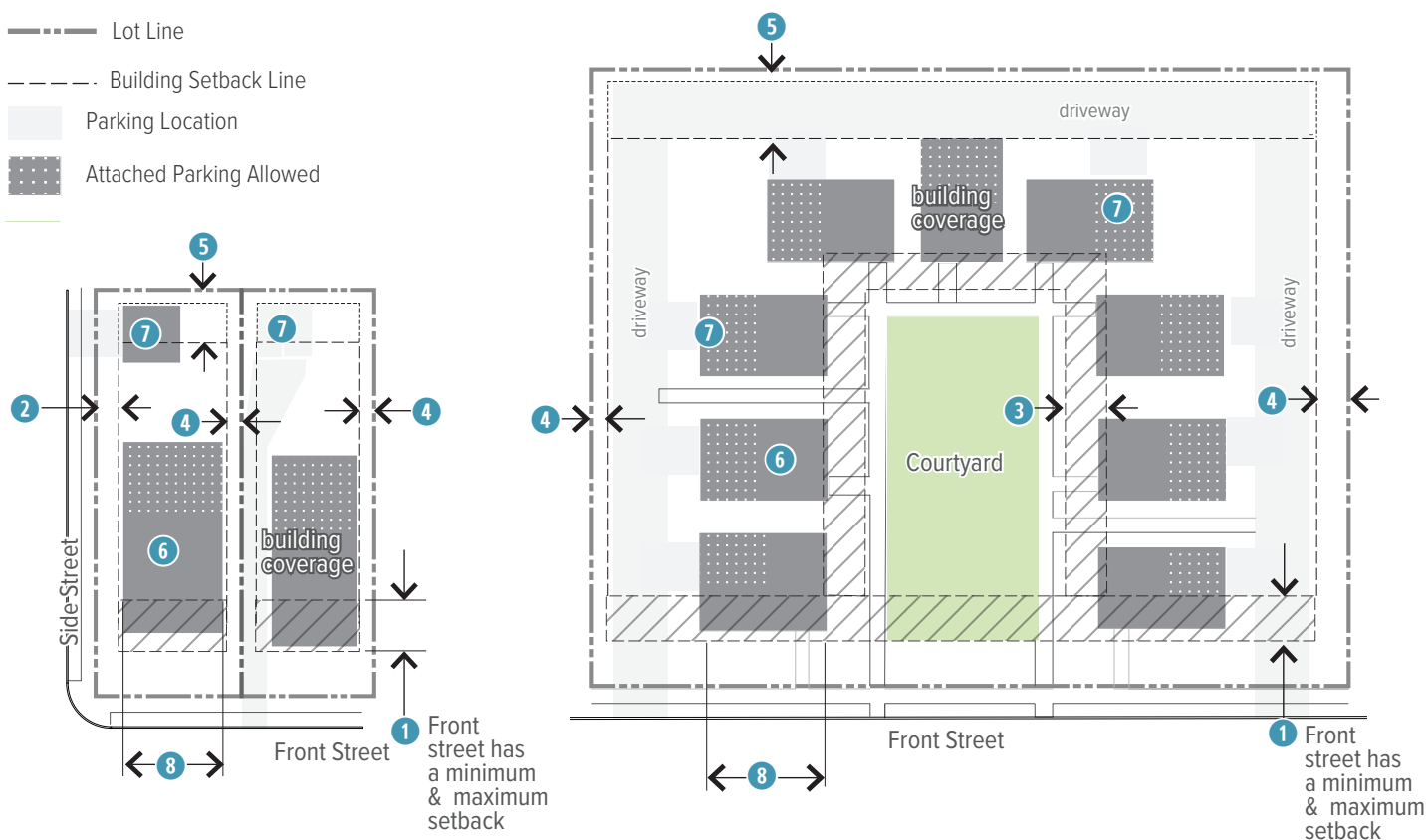
Figure 16. Cottage House Diagrammatic Plan
